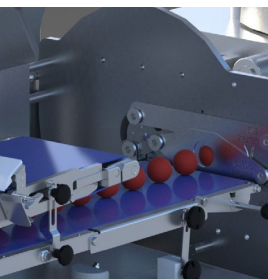
↑ Forming principle: Free forming and optional flattening
