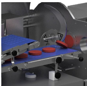
↑ Forming principle: Forming and cutting
